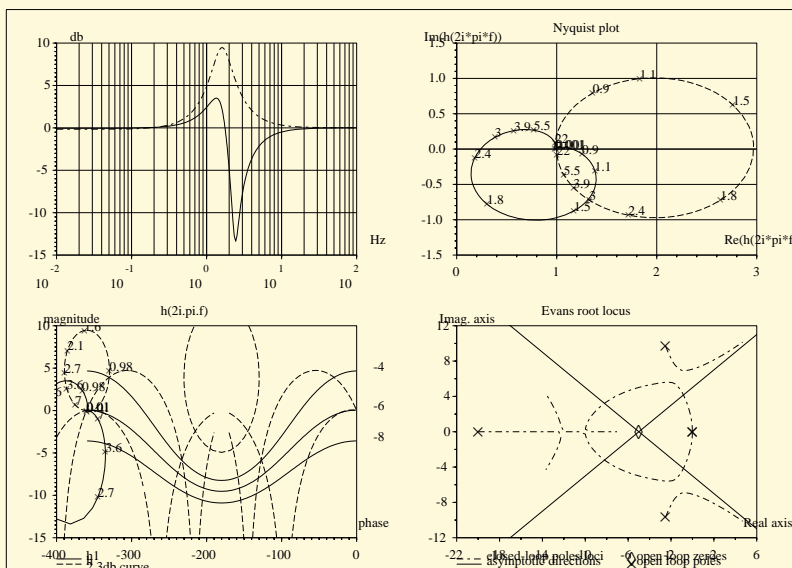
圖 6.8: Some Plots in Automatic Control
