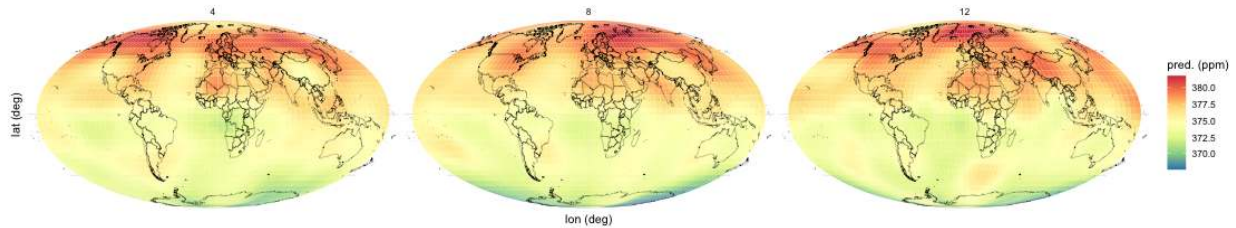
Figure 17: Prediction of Y_P in ppm on 04, 08, and 12 May 2003 obtained with FRK on the AIRS data.
