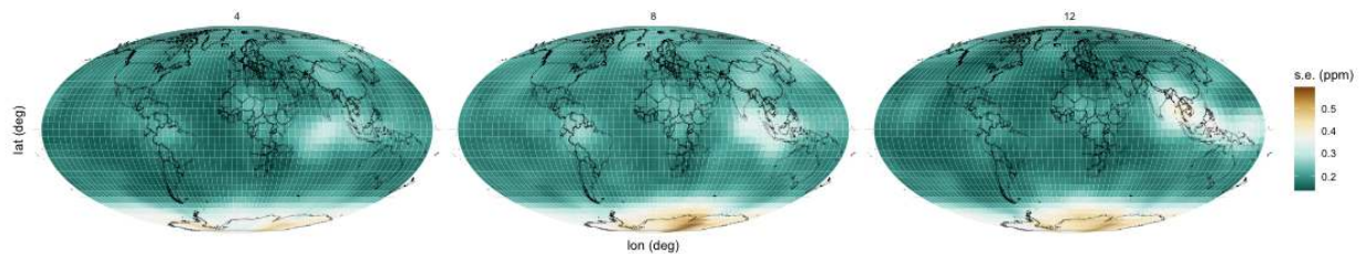
Figure 18: Prediction standard error of Y_P in ppm on 04, 08 and 12 May 2003 obtained with FRK on the AIRS data.
